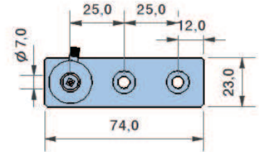
SUPORTE . SUPPORT G
