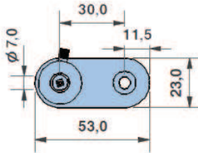
SUPORTE . SUPPORT F
