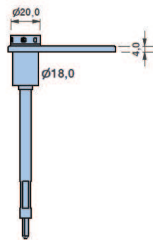
SUPORTE . SUPPORT G
