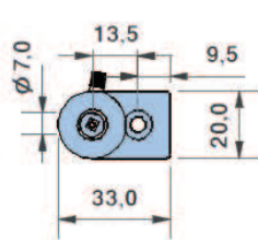
SUPORTE . SUPPORT F
